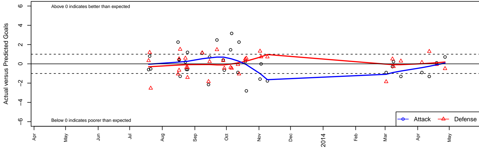
Thelo Spartans B02 Dots are actual minus expected GF (blue circles) and GA (red triangles). Blue line is smoothed change in attack strength. Red is smoothed change in defense strength.
